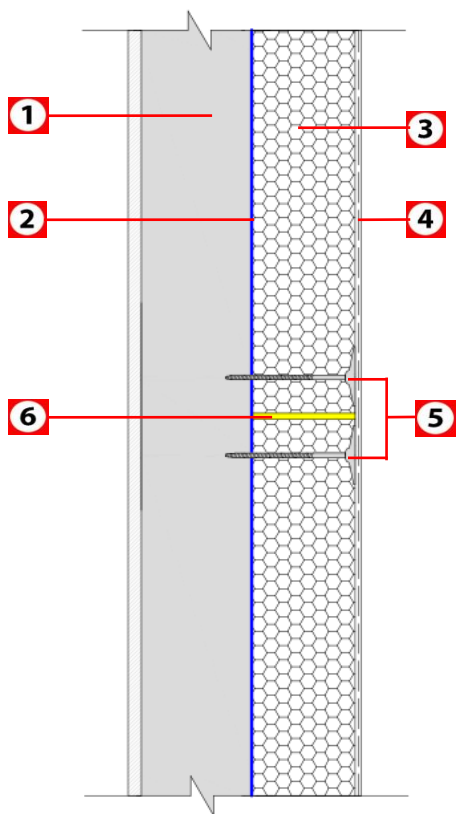
Horizontal Joints – Section View
