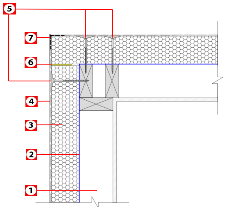
External Corner – Plan View
