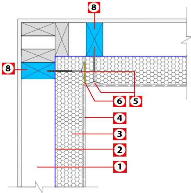
Internal Corner – Plan View
